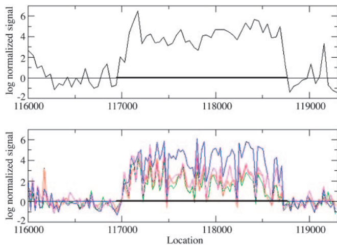
Fig. 2. Hybridization intensities for the gene At1g01300, encoding an aspartyl protease family protein previously verified by EST and cDNA, are shown here. (Upper) This study. (Lower) Previous study (11). Red, flower; green, root; blue, suspended cell; magenta, cells in the presence of light. The gene is located on Watson strand of chromosome 1 and has only one exon marked by solid black line near y = 0 . For long exons, this study obtained signals above cutoff for all or most probes, whereas the signals measured by the previous study more often fell below the cutoff. This result could be due to the difference in choices of probe lengths or to other differences in hybridization protocol between the two experiments.
