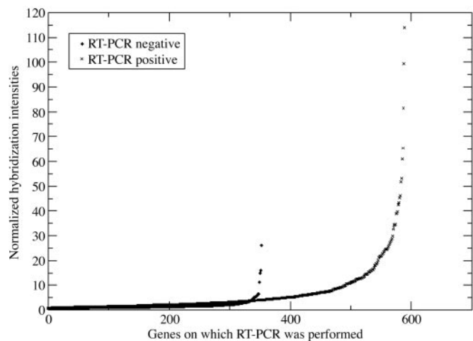
Fig. 4. Plot of hybridization intensities (T87 cell line) for the 594 RT-PCR positive (X) and 353 RT-PCR negative (◆) genes. Strong hybridization intensities observed for some RT-PCR negative genes (near gene no. 350) were artifacts due to ORF-based primer choices. Seventeen of 20 RT-PCR negative genes in this region were later confirmed positive by a measurement that chose different sets of primers.
